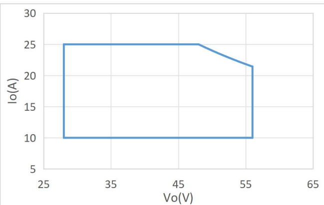
I/V Operating Area
